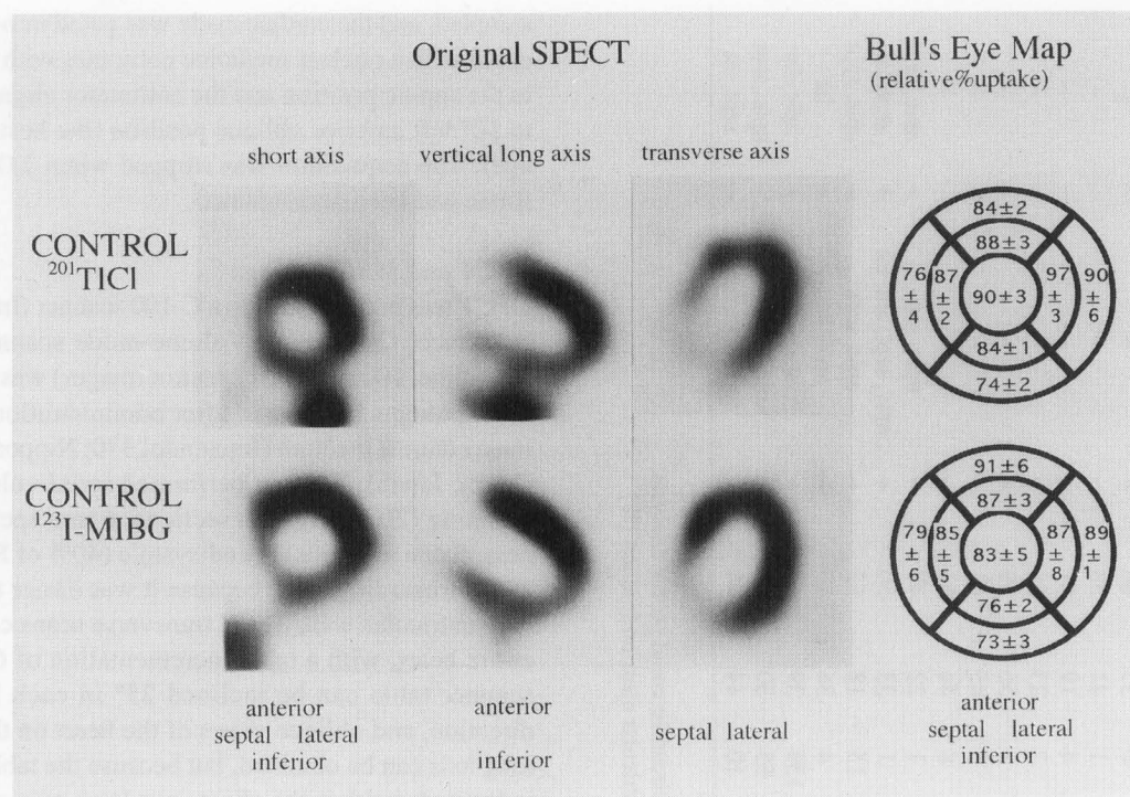
Fig. 3 ^{201}\text{TlCl} and ^{123}\text{I-MIBG} images of a representative case, and bull's eye map of the relative ^{123}\text{I-MIBG} uptake in the control group. There is a homogeneous distribution of ^{201}\text{TlCl} and ^{123}\text{I-MIBG} . Values are given as mean \pm SD.
