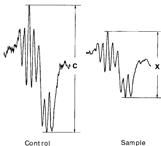
Fig. 1 A typical ESR spectrum of non-radioactive Cu-PTSM. Reduction rate (%) of Cu-PTSM was calculated as (C - X)/C \times 100 . C: ESR signal of the control, X: ESR signal of the sample.
