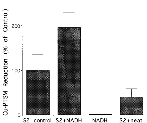
Fig. 3 The Cu-PTSM reduction ability of the tumor S2 fraction (microsome/cytosol), S2 with NADH, NADH alone and S2 after heat treatment. Data are the average of four experiments.
