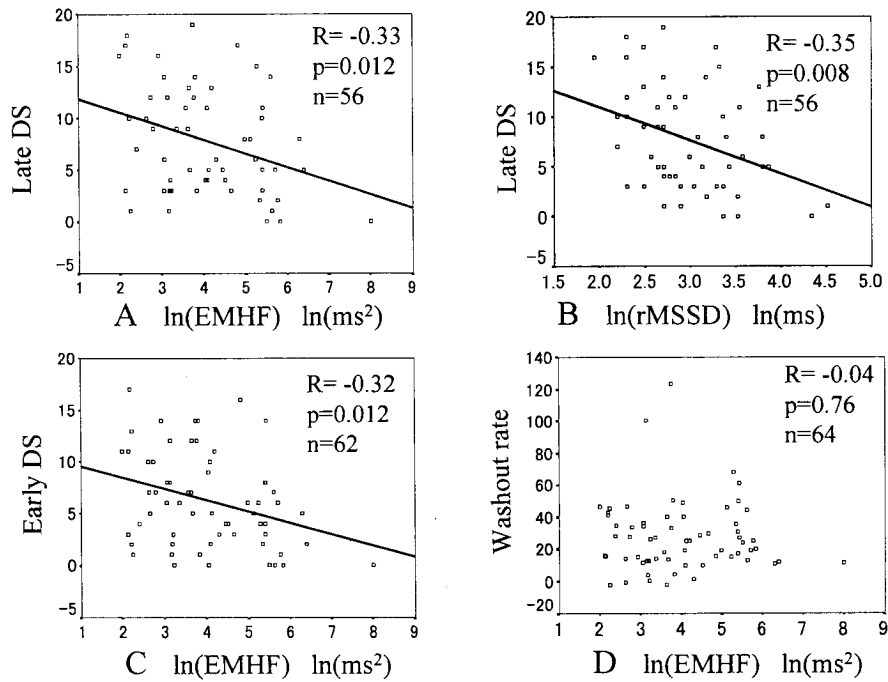
Fig. 1 In the total population the relation between sympathetic parameters of MIBG and parasympathetic parameters of HRV. A: the relation between late DS and EMHF in the total population. B: the relation between late DS and rMSSD in the total population. C: the relation between early DS and EMHF in the total population. D: the relation between washout rate and EMHF in the total population. EMHF, early morning high-frequency power (from 2 a.m. to 5 a.m.).
