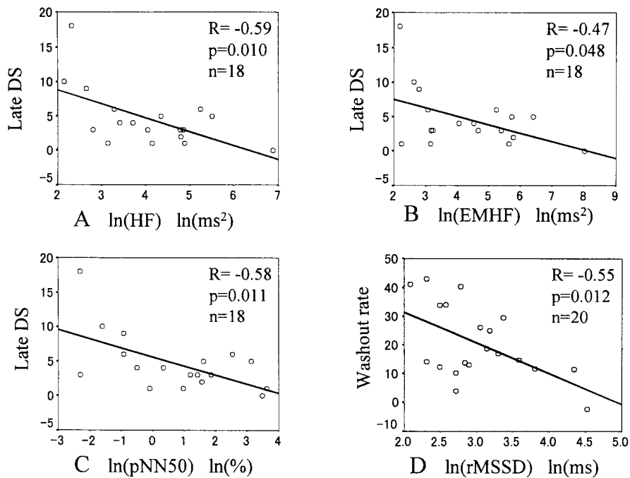
Fig. 2 In the selected population the relation between sympathetic parameters of MIBG and parasympathetic parameters of HRV. A: the relation between late DS and HF in the selected population. B: the relation between late DS and EMHF in the selected population. C: the relation between late DS and pNN50 in the selected population. D: the relation between washout rate and rMSSD in the selected population. EMHF, early morning high-frequency power (from 2 a.m. to 5 a.m.); HF, high-frequency power; pNN50, proportion of adjacent normal RRs more than 50 msec different; rMSSD, root-mean square of difference of successive RRs.
