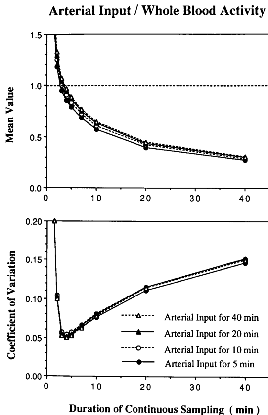
Fig. 5 The results of simulation study for estimation of arterial input function from the total blood activity. The ratio of the arterial input to the activity in the total arterial blood sample (upper figure) decreased with time due to the increment of hydrophilic metabolites in blood. The coefficient of variation (lower figure) showed minimum values (approximately 5%) between 3 and 5 min.
