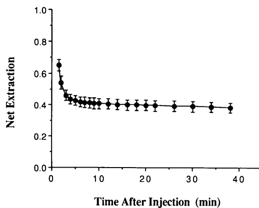
Fig. 3 Temporal changes of net extraction calculated by brain SPECT counts and arterial input function using rCBF measured by PET as a reference (mean \pm s.d. of 6 subjects). The net extraction showed a rapid decrease within 5 min but the value was stable thereafter.
