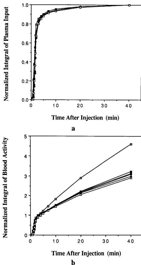
Fig. 4 a. Temporal changes of the integral of arterial input function in 6 subjects. The value was normalized by the total input activity for 40 min in each subject. The shape was quite similar among the subjects. b. Temporal changes of the integral of total blood activity in 6 subjects. The value was also normalized by the total input activity for 40 min in each subject. The variation among the subjects may be due to the different clearance of hydrophilic metabolites.
